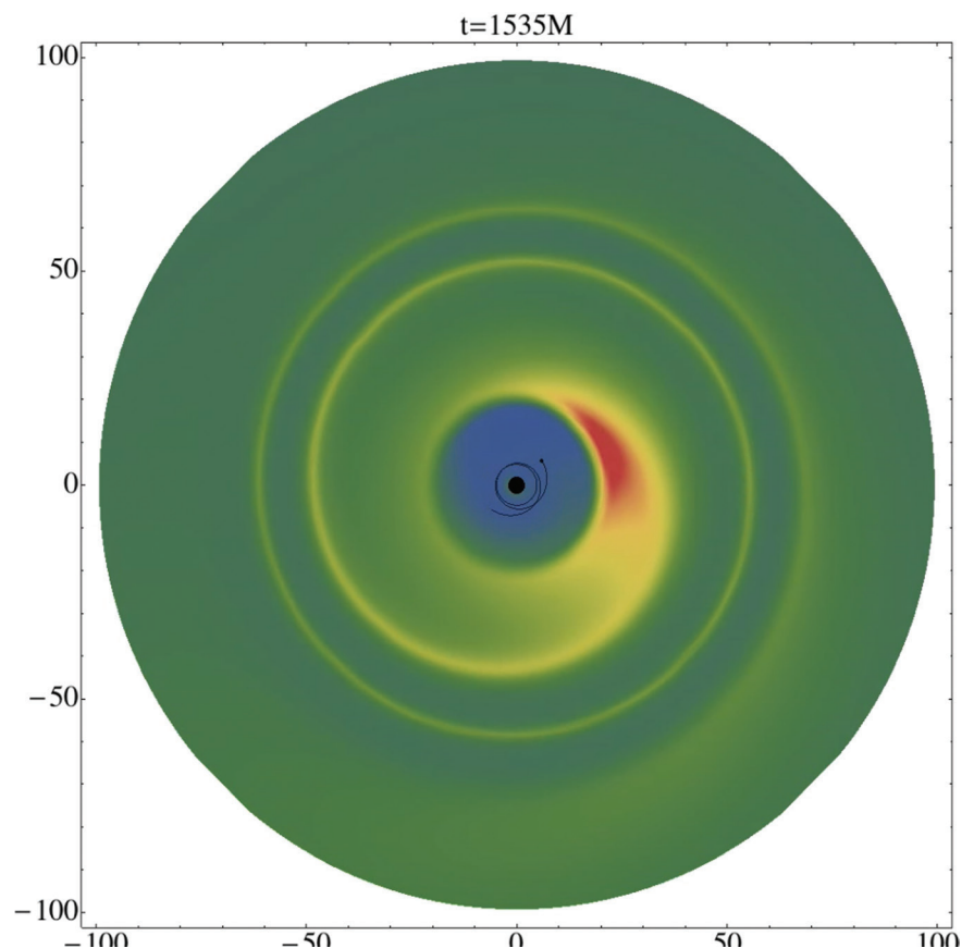
Equatorial snapshot of the scalar field produced by a scalar charge in orbit around a black hole. The central black dot shows the black hole. The smaller black dot shows the current location of the scalar charge and the line trailing it shows a part of the previous trajectory. Notice the spiral pattern in the wave traveling outwards.
